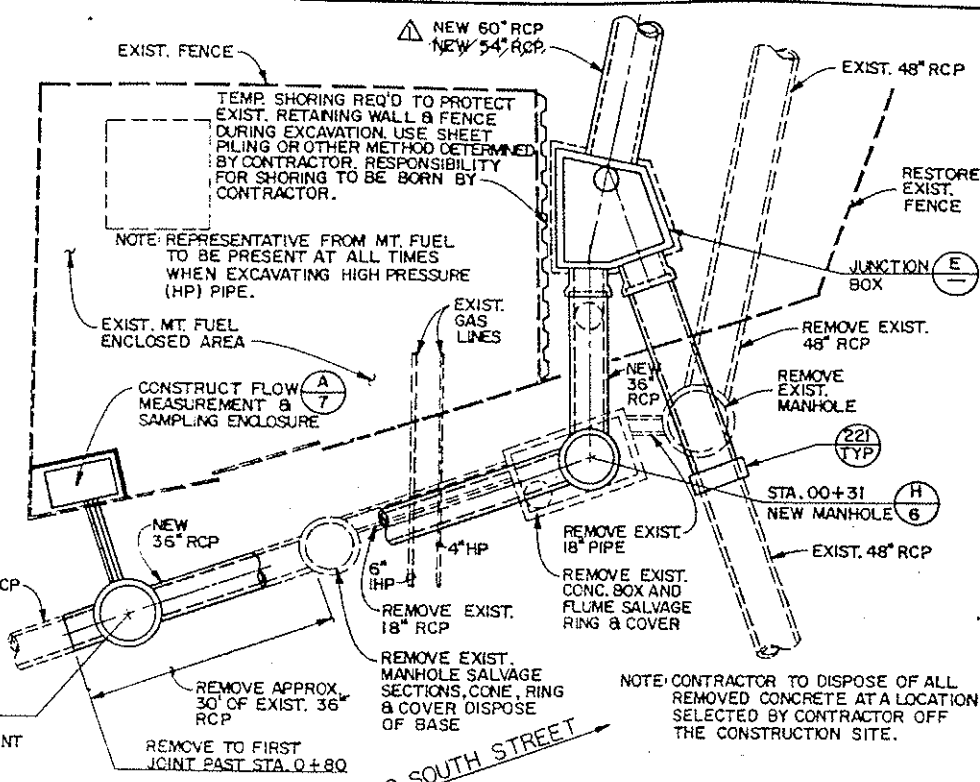
D DEMOLITION PLAN VIEW SCALE: 1" = 10'
