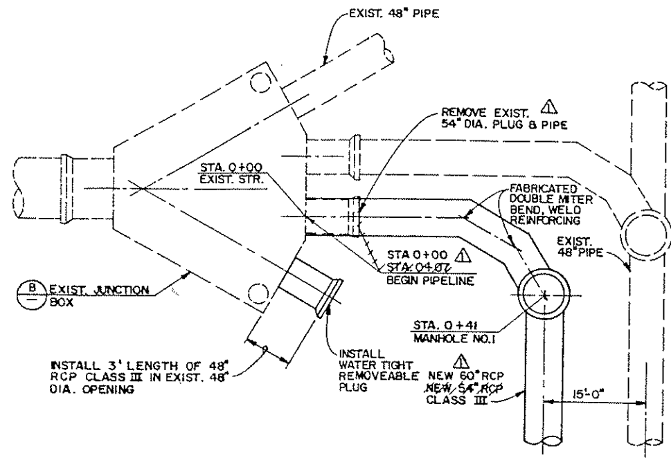
A JUNCTION BOX CONNECTION SCALE: 1" = 10'
