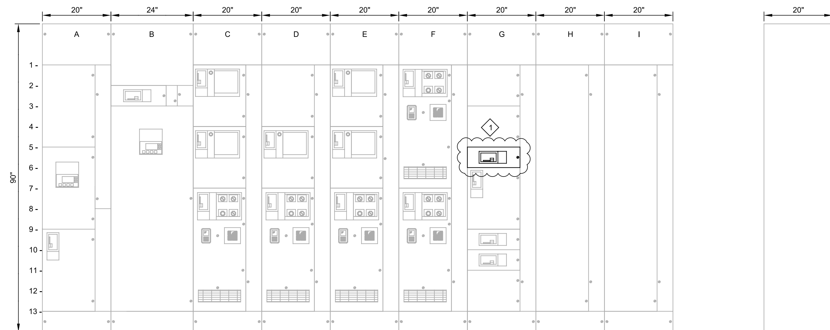
FRONT VIEW
